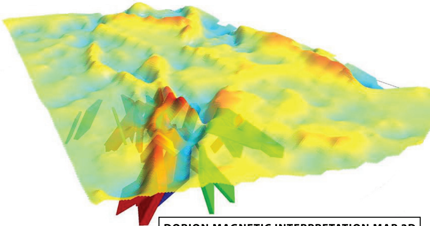
DORION MAGNETIC INTERPRETATION MAP 3D
